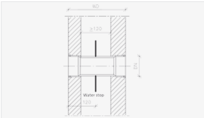
Transwand DM in an element wall
